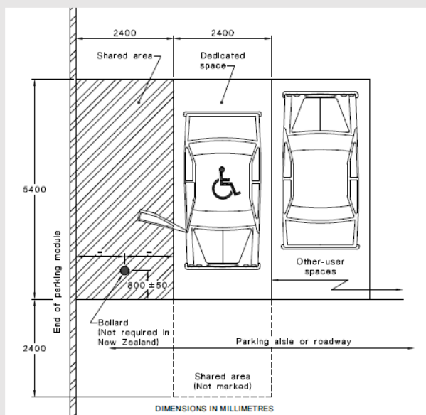
FIGURE 2.2 EXAMPLE OF AN ANGLE PARKING SPACE WITH SHARED AREA ON ONE SIDE ONLY—DIMENSIONS FOR AUSTRALIA ONLY*
